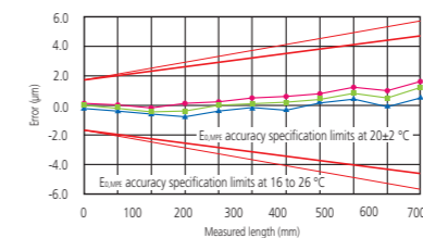
Graph showing the effectiveness of temperature compensation
